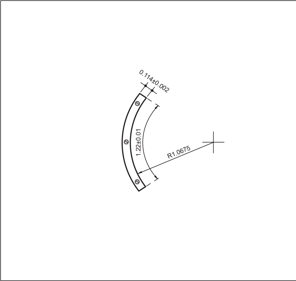
Shot Put stop board (1983/84 specifications, dimensions in m) (Acceptable under Rule 188.2 Note)
